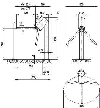
BAR-SKR
